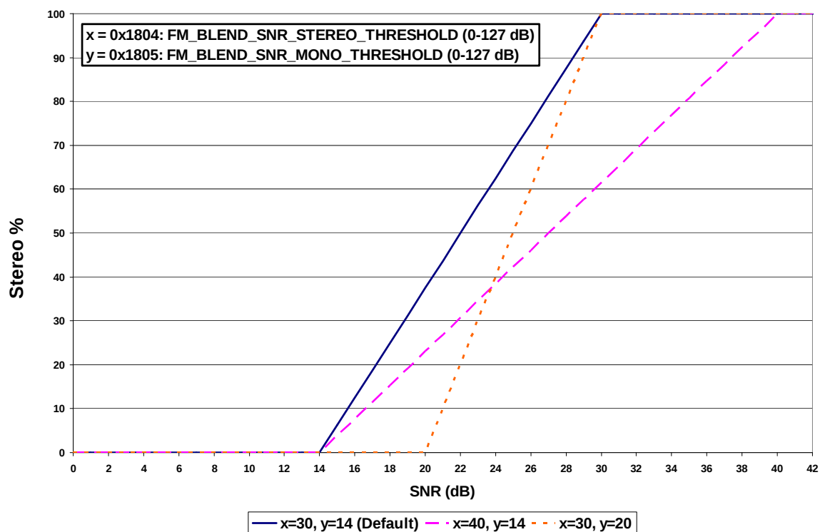
Figure 5. SNR Blend
