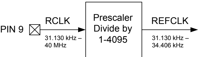
Figure 16. REFCLK Prescaler
